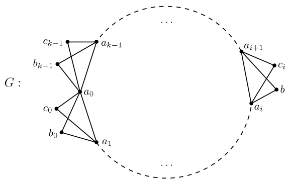
Fig. 3. A circular-arc graph G with 3k vertices and 2^{O(k)} different vertex sets that provide a longest path of G .
