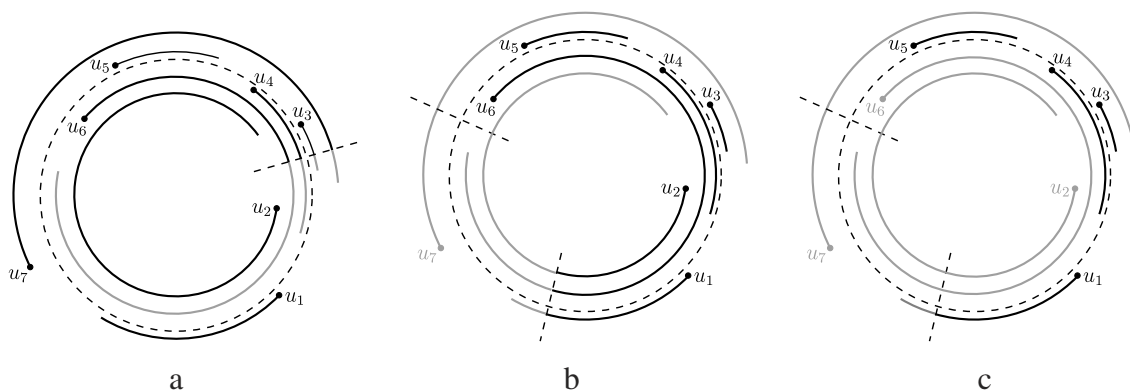
Fig. 2. The circular-arc representations of three (not necessarily induced) subgraphs of the circular-arc graph G of Fig. 1(a): (a) the interval graph G_{u_3} = G_3(2) , (b) the interval graph G_1(6) , and (c) the interval graph G(1, 6) .
