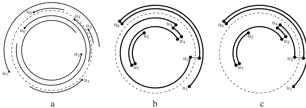
Fig. 1. (a) A circular-arc representation of a circular-arc graph G with the right-end circular ordering \pi = (u_1, u_2, u_3, u_4, u_5, u_6, u_7) , (b) a path-arc representation P_{\text{arc}} of the path P = (u_1, u_6, u_2, u_4, u_3, u_7, u_5) of G , which covers all the circle, and (c) another path-arc representation of P , which does not cover all the circle.
